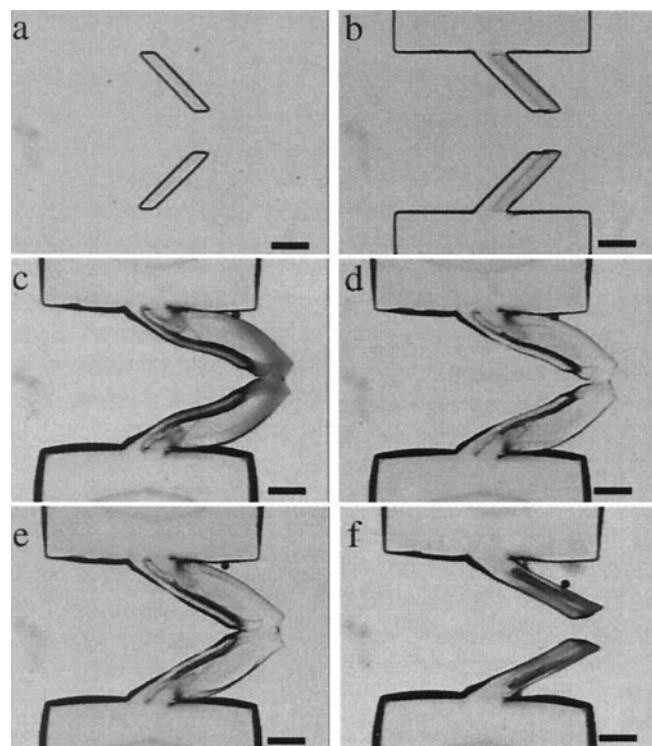
Fig. 6. A biomimetic valve based on bistrip hydrogel. (a) After simultaneous polymerization of the pH-sensitive strips. The hydrogel composition is the same as that described in Fig. 4e. (b) After polymerization of the non-pH-sensitive strips to form the bistrip hydrogel valve with anchor. The prepolymer mixture for the non-pH-sensitive hydrogel consists of HEMA, EGDMA (1.0 wt %), and Irgacure 651 (3.0 wt %). (c) When exposed to basic solution, the bistrip hydrogel expands and curves to form a normally closed valve. The bistrip valve can be pushed open (d) to allow flow in one direction (from left to right) while restricting flow in the opposite direction (e). (f) When exposed to acidic solutions, the valve is deactivated, returning to the permanently open state. (Bars = 500 \mu\text{m} .)
